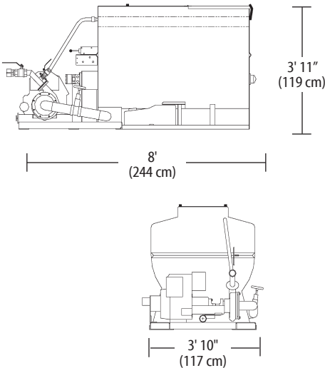
T30 SKID MOUNT
